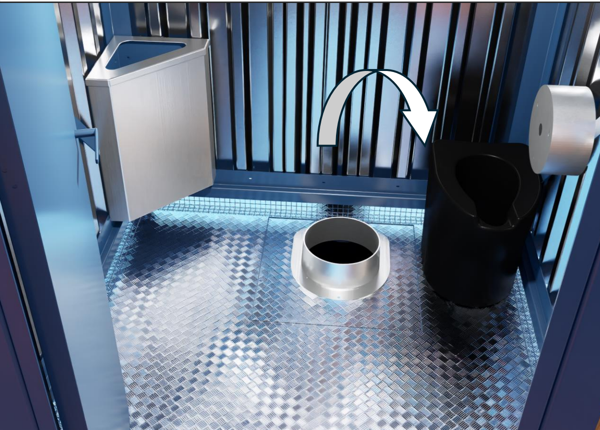
- Step 1: Remove the bowl
